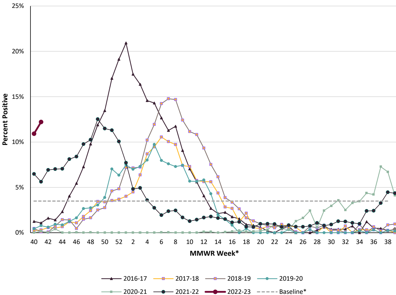
Figure 4. Percentage of Respiratory Specimens Testing Positive for Respiratory Syncytial Virus (RSV) at LAC Sentinel Surveillance Laboratories by Season, 2016-17 Through 2022-23
