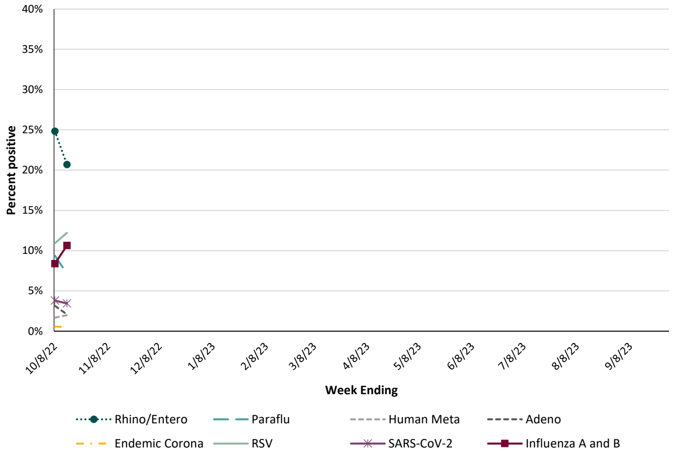
Figure 3. Percentage of Respiratory Specimens Testing Positive by Viral Etiology, Los Angeles County Sentinel Surveillance Laboratories, 2022-23 Influenza Season
