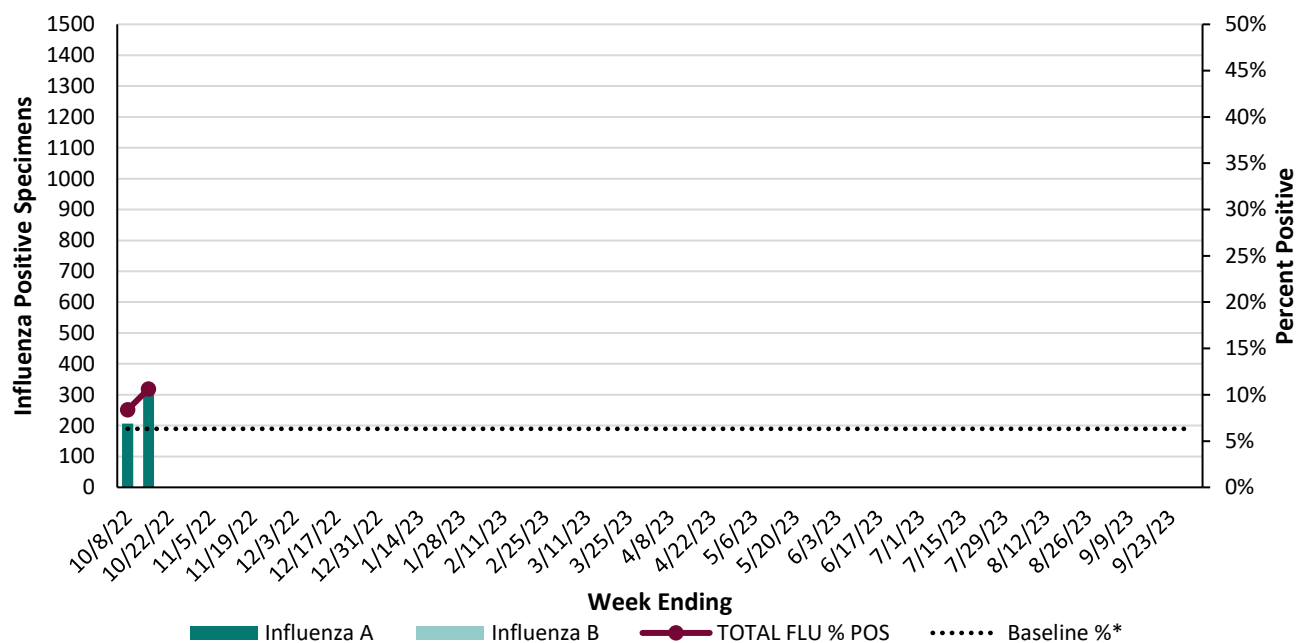
Figure 1. Respiratory Specimens Tested and Percent Positive for Influenza Virus by LAC Sentinel Surveillance Laboratories, 2022-23 Influenza Season
