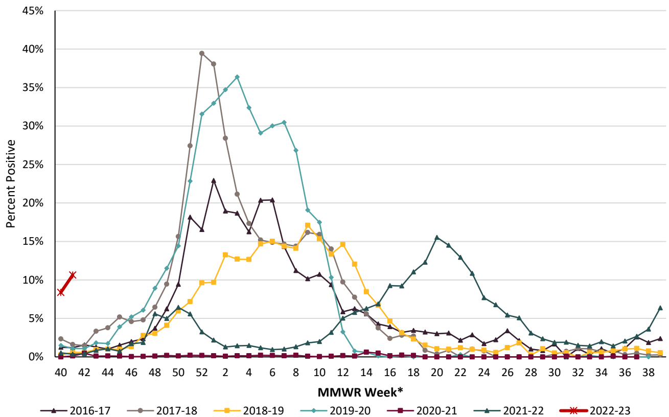
Figure 2. Percentage of Respiratory Specimens Testing Positive for Influenza at LAC Sentinel Surveillance Laboratories by Season, 2016-17 Through 2022-23
