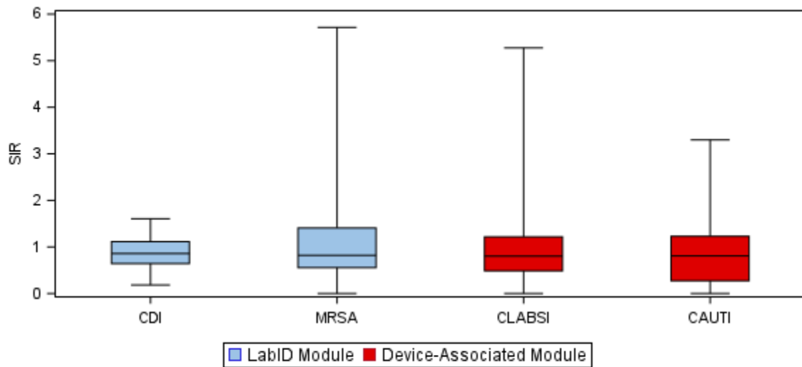
Figure 2: Boxplots of Healthcare Facility-Onset Infection Rates, General Acute Care Hospitals, L.A. County, 2018
